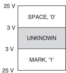
Figure 7. RS-232 Signals
