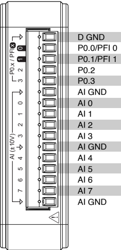
Figure 1. USB-6000 Pinout
