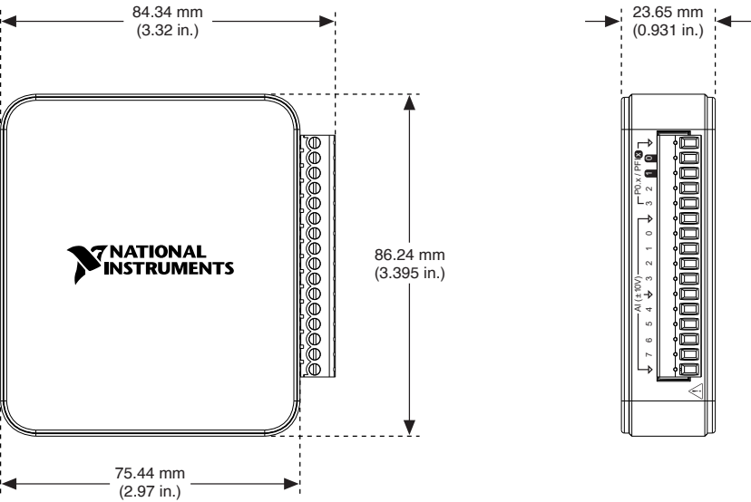
Figure 2. USB-6000 Dimensions
