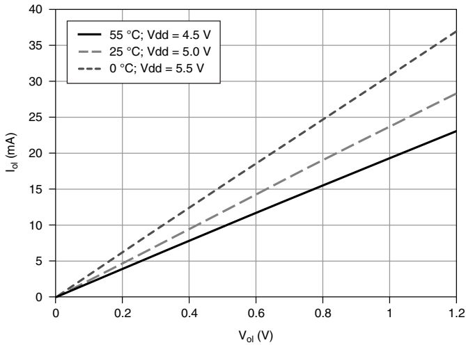
Figure 4. PFI <0..15>/P0.<0..15>: I_{ol} versus V_{ol}
