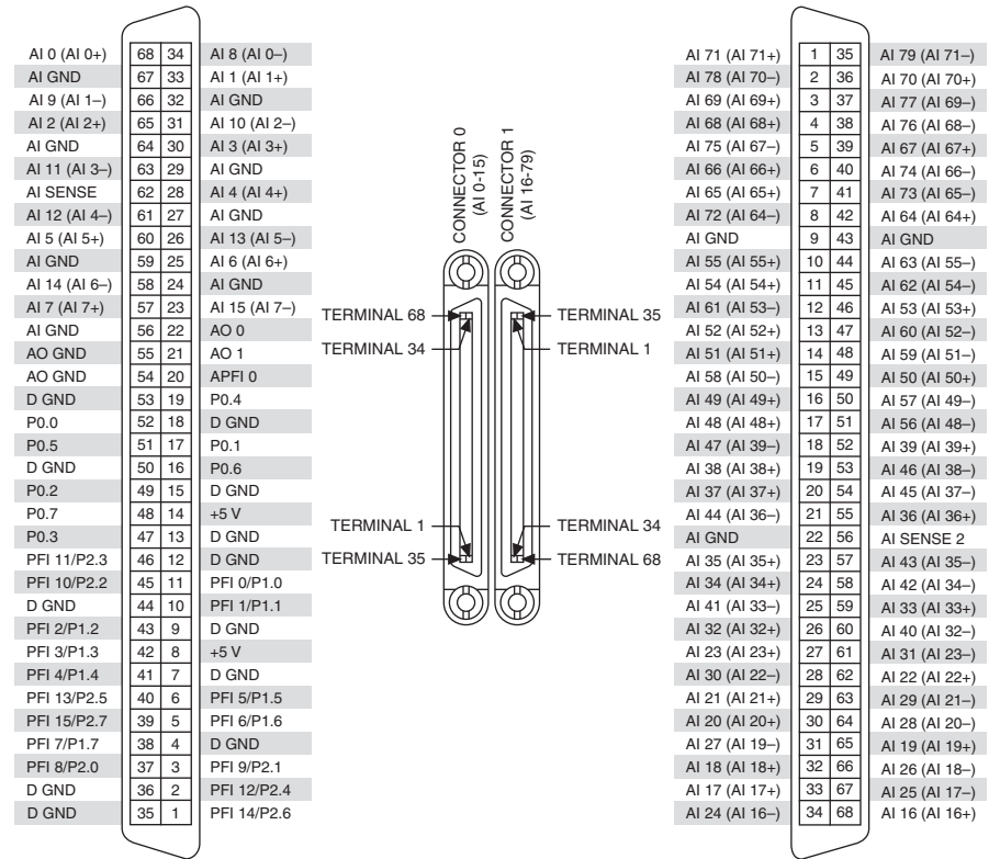
Figure A-19. PCI/PXI-6255 Pinout
