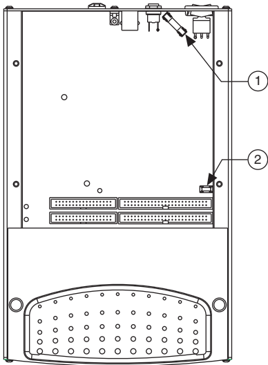
Figure 1-8. USB-62xx Screw Terminal Fuse Locations
