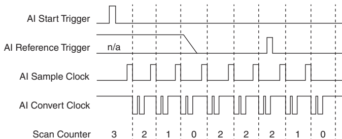
Figure 4-15. Pretriggered Data Acquisition Example
