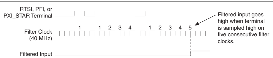
Figure 8-3. Filter Example
