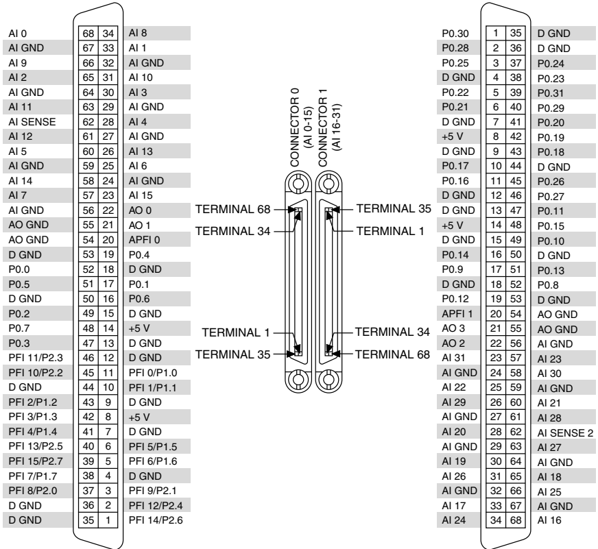
Figure 9. NI PCI/PCIe/PXI/PXIe-6259 Pinout
