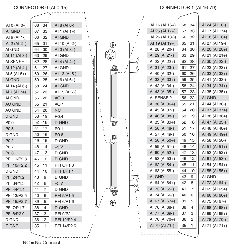
Figure A-9. USB-6225 Mass Termination Pinout
