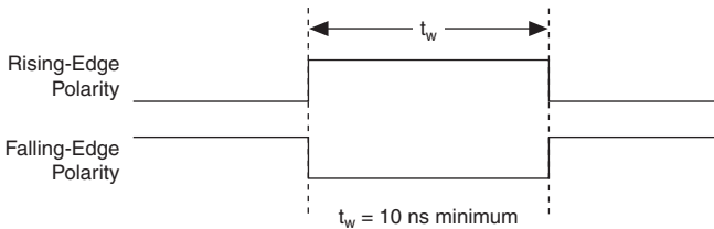
Figure 3-6. ao/SampleClock Timing Requirements
