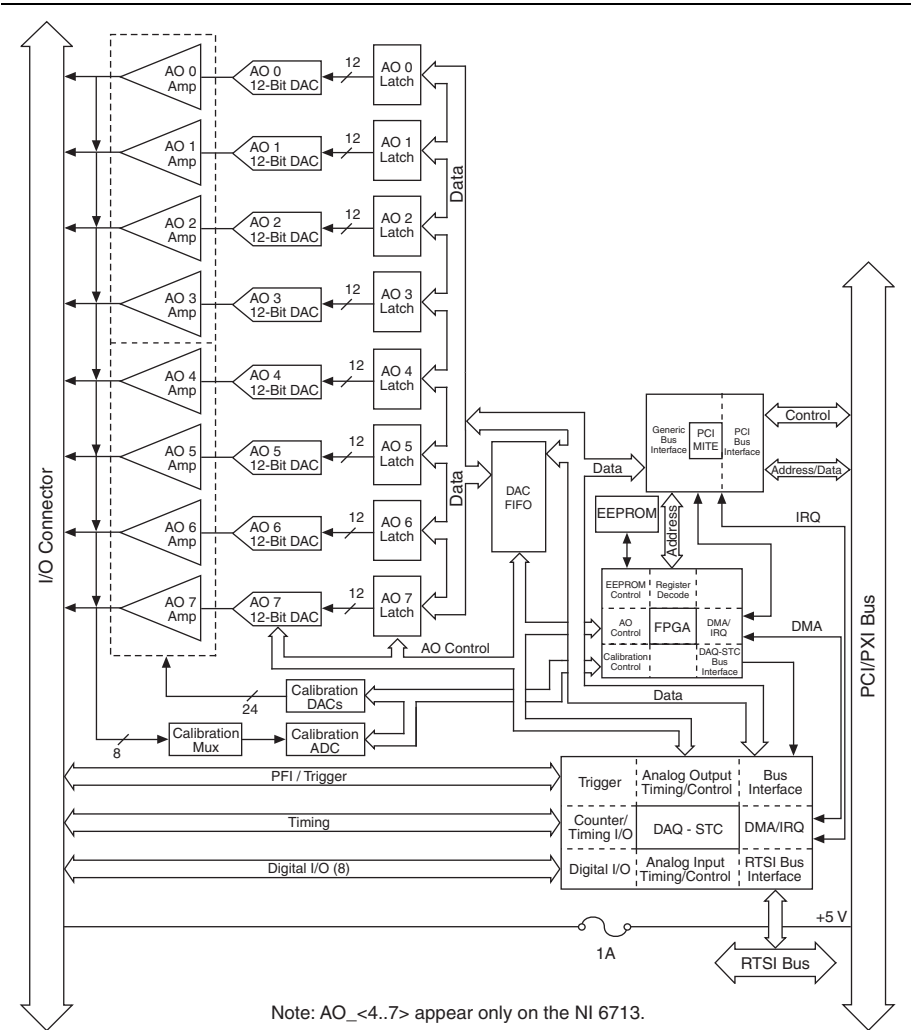
Figure A-1. NI 6711/6713 Block Diagram
