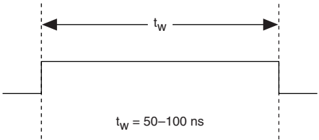
Figure 3-5. PFI 6/AO START TRIG Timing Behavior
