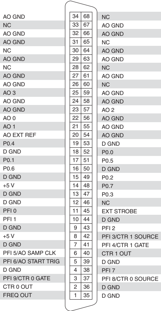
Figure 2-1. NI 6711/6731 68-Pin AO I/O Connector Pinout
