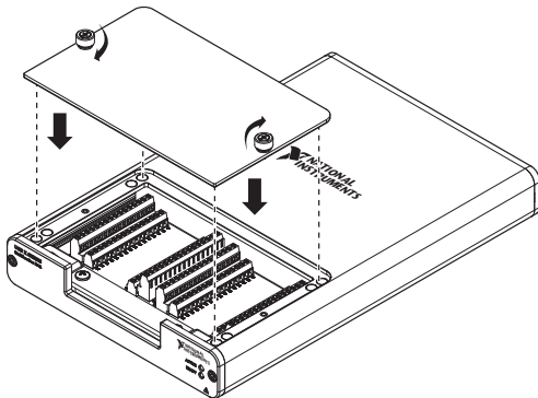
Figure 1. Installing the Locking Lid
