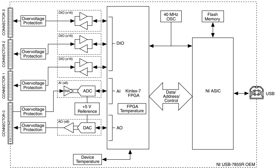
Figure 1. USB-7855R OEM Device Block Diagram
