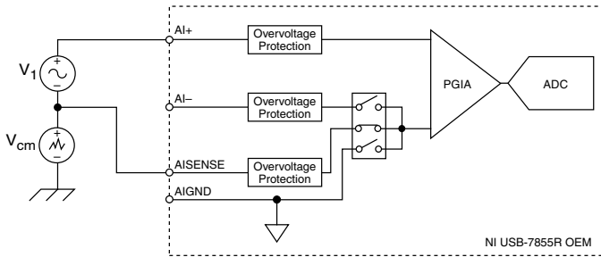
Figure 4. Connecting Non-Referenced Single-Ended Signals to the USB-7855R OEM Device
