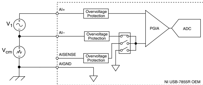
Figure 5. Connecting Grounded Differential Signals to the USB-7855R OEM Device
