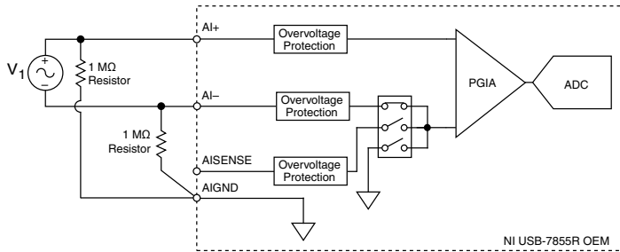
Figure 6. Connecting Floating Differential Signals to the USB-7855R OEM Device
