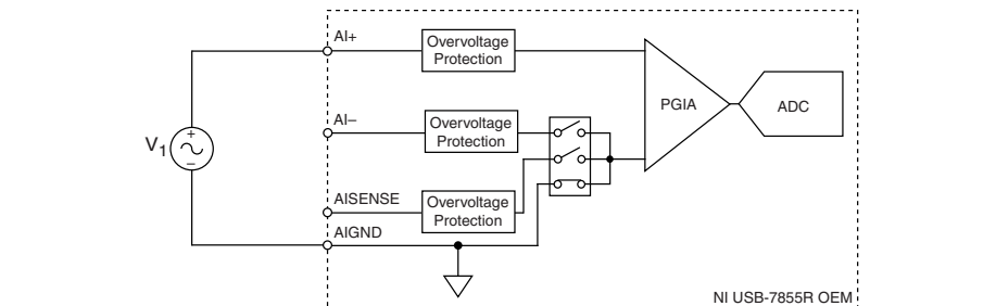
Figure 3. Connecting Referenced Single-Ended Signals to the USB-7855R OEM Device
