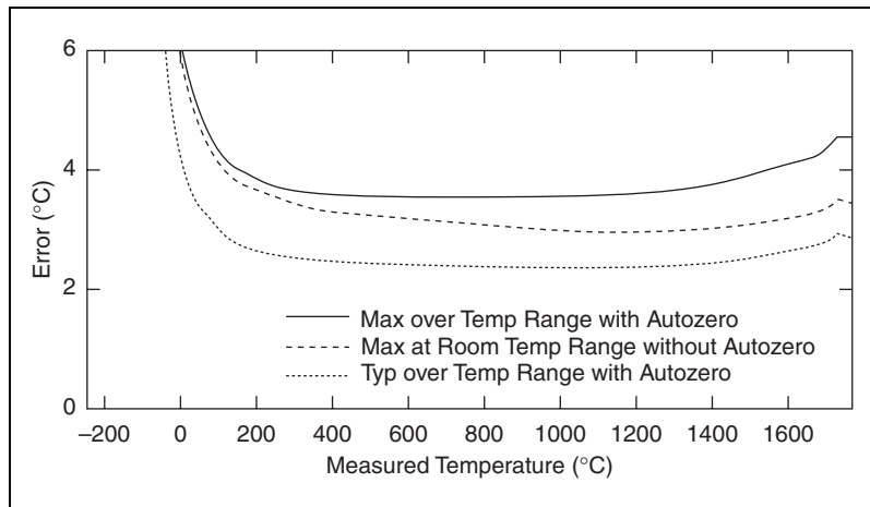
Figure 14. Type R and S Errors
