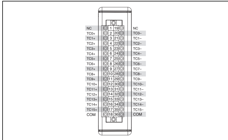
Figure 7. NI USB-9213 Terminal Assignments
