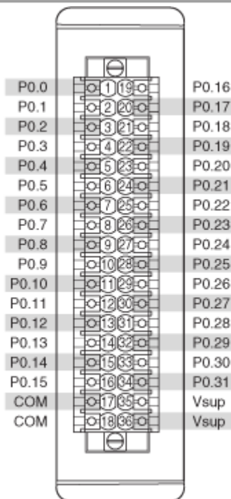
NI 9476 Spring Terminal
