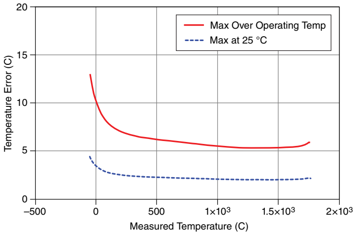
Figure 4. Temperature Error of Type S Thermocouple
