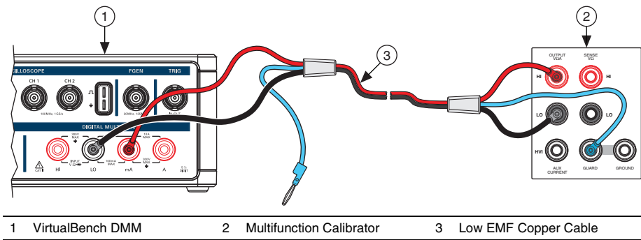
Figure 6. Cable Connections for AC Current Ranges \leq 50 mA
