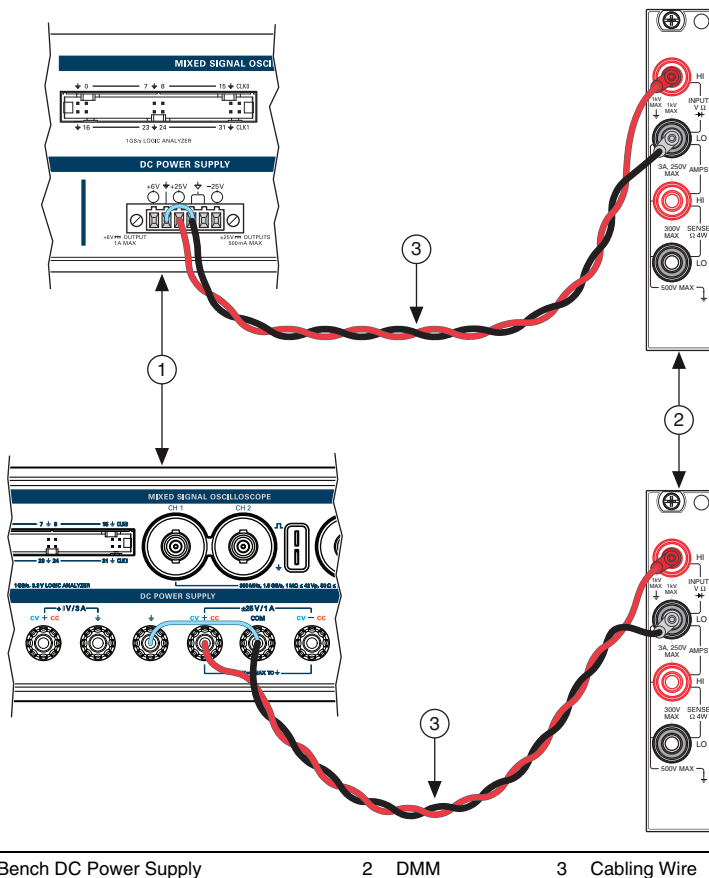
Figure 30. Cable Connections For +25 V Voltage Programming Accuracy Verification
