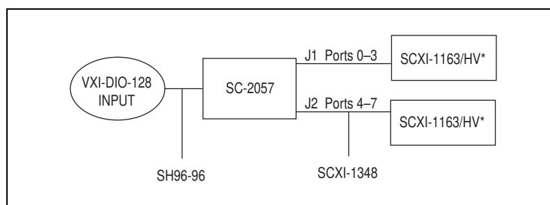
Figure 9-6. Input Connections with the SCXI-1162/HV
