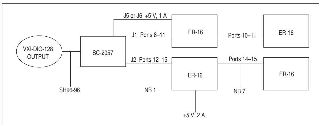
Figure 9-3. Output Connections with the ER-16
