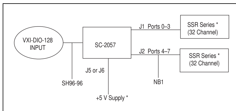
Figure 9-7. Input Connections with the 32-Channel SSR Backplane
