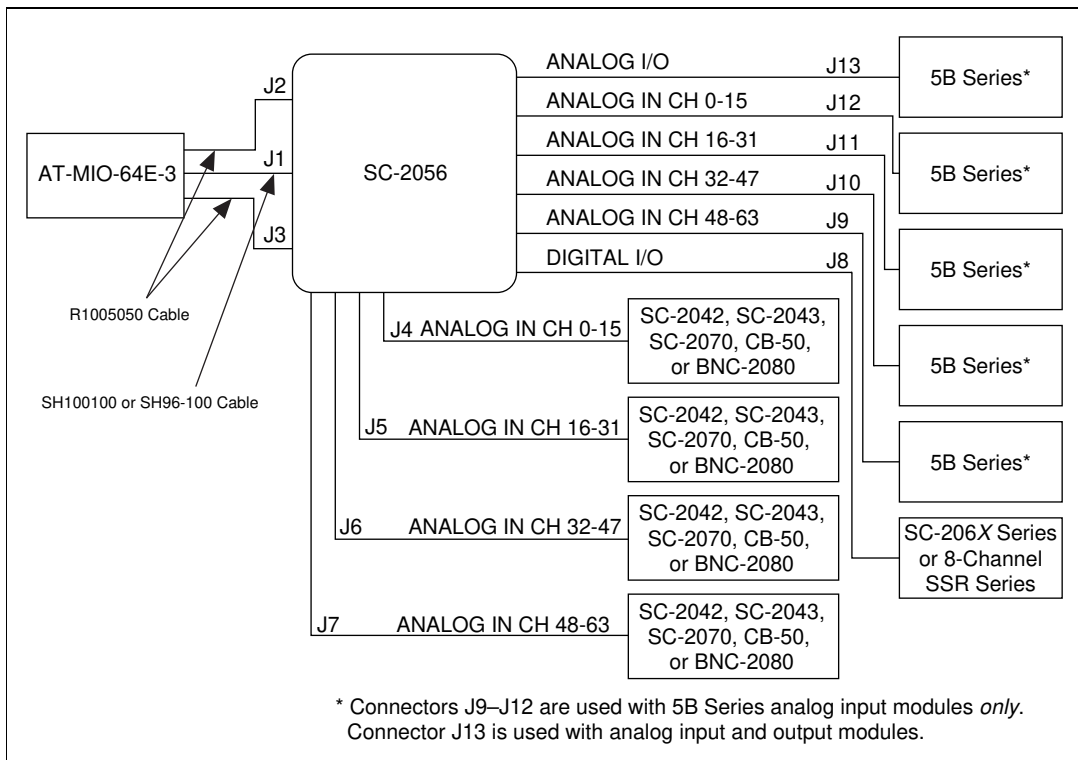
Figure 8-2. SC-2056 Connections
