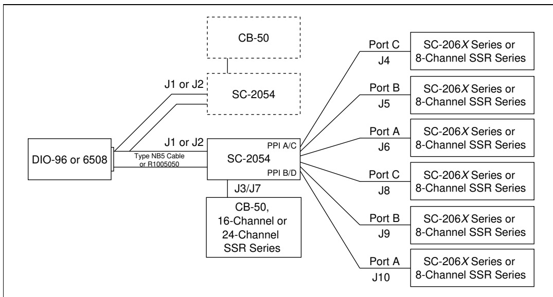
Figure 6-2. SC-2054 Connections
