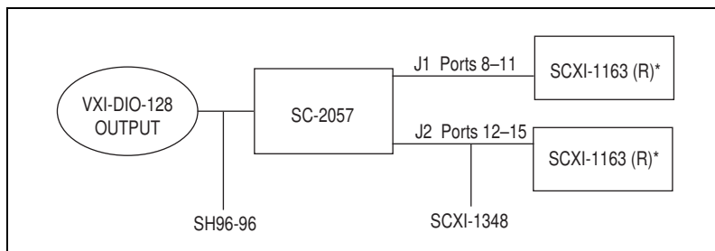
Figure 9-2. Output Connections with the SCXI-1163/R
