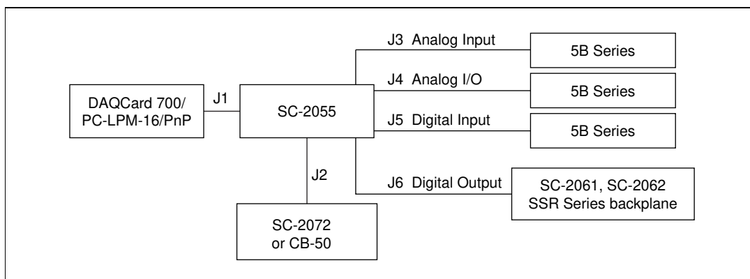
Figure 7-2. SC-2055 Connections
