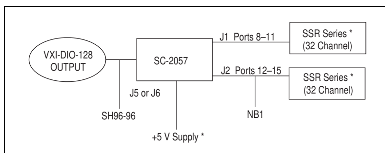
Figure 9-4. Output Connections with the 32 Channel SSR Backplane
