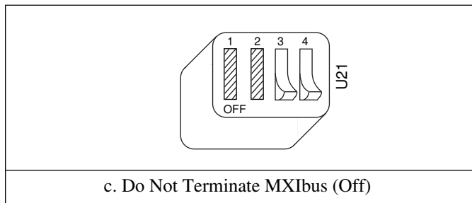
Figure 3-4. MXIbus Termination
