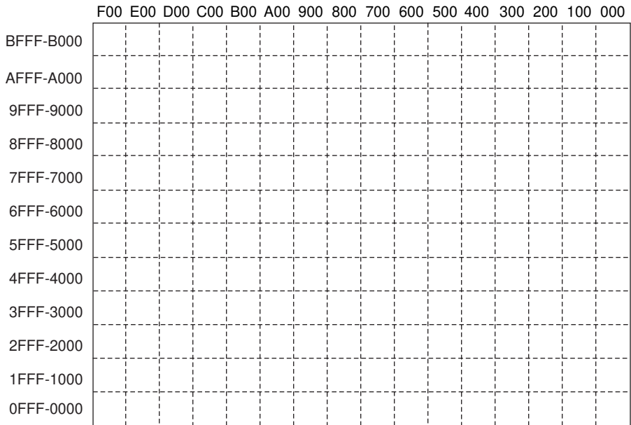
Figure 5-24. A16 Space Address Map Diagram for Your VMEbus/MXibus System
