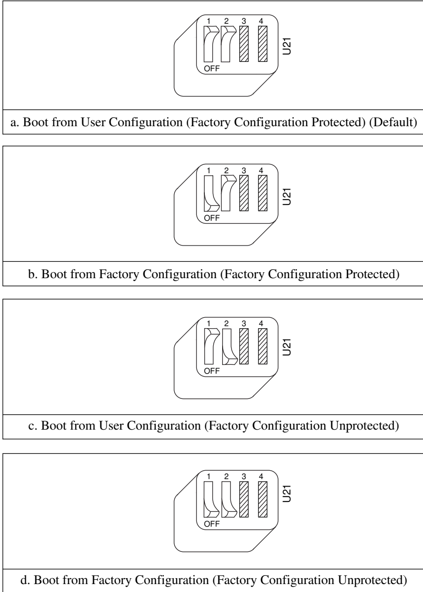
Figure 3-5. EEPROM Operation
