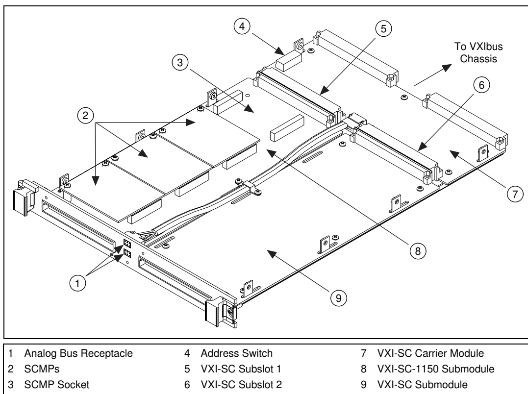
Figure 1-1. VXI Signal Conditioning System
