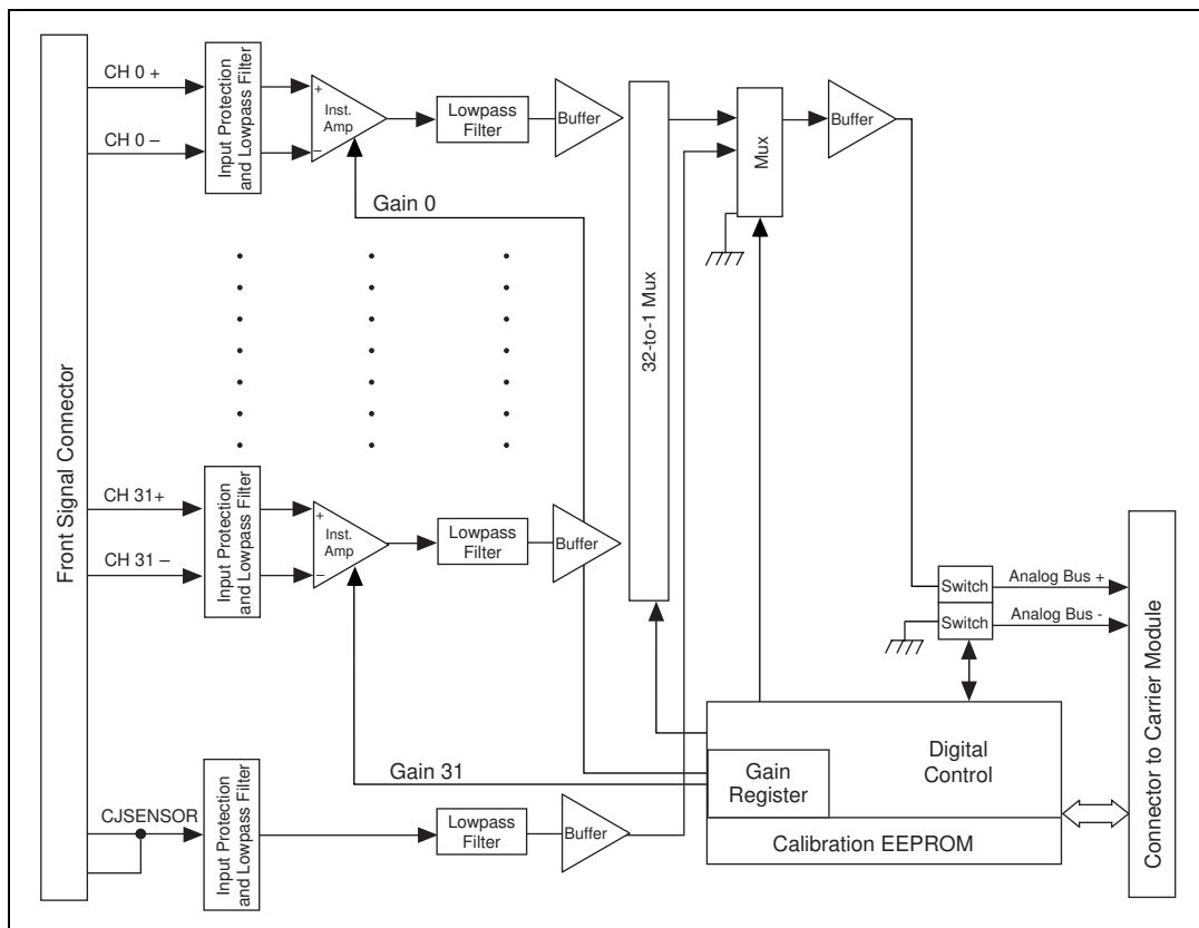
Figure 4-1. VXI-SC-1102/B/C Block Diagram
