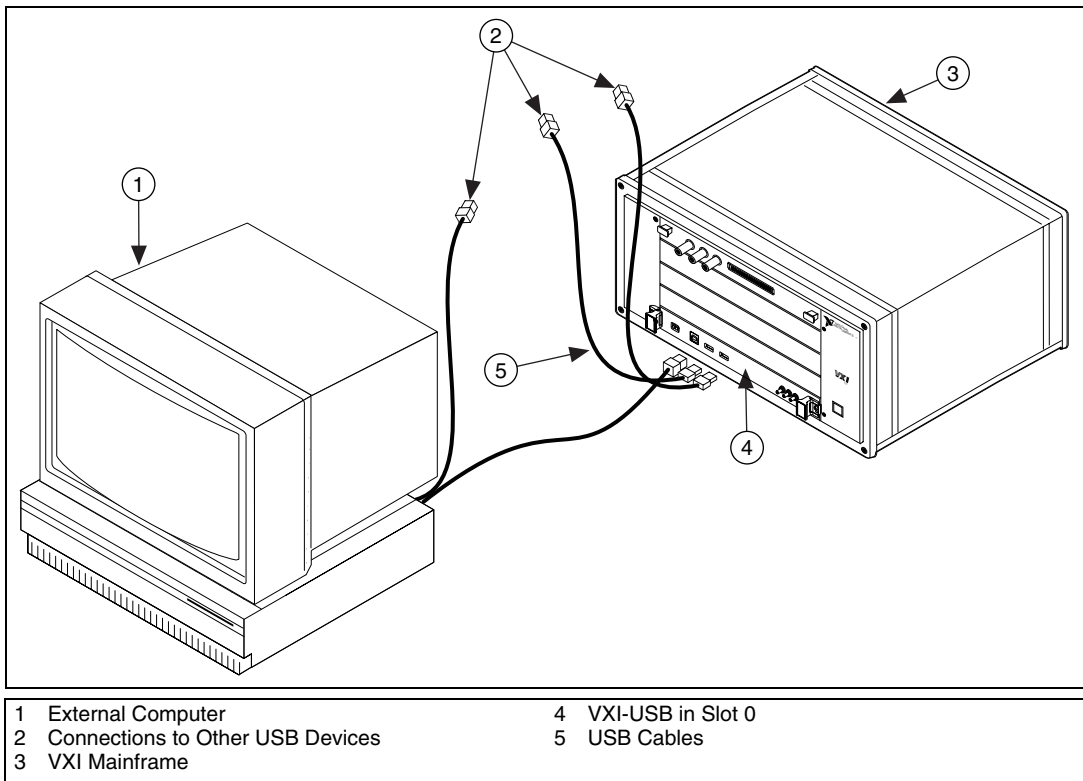
Figure 2-2. USB System
