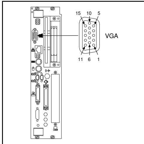
Figure D-3. VGA Connector Location and Pinout
