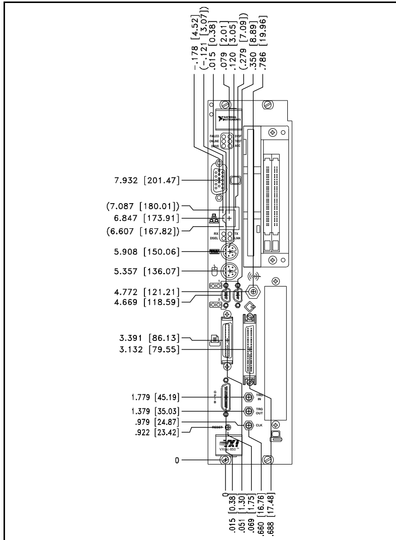
Figure D-1. VXIpc-850 Front Panel Layout and Dimensions
