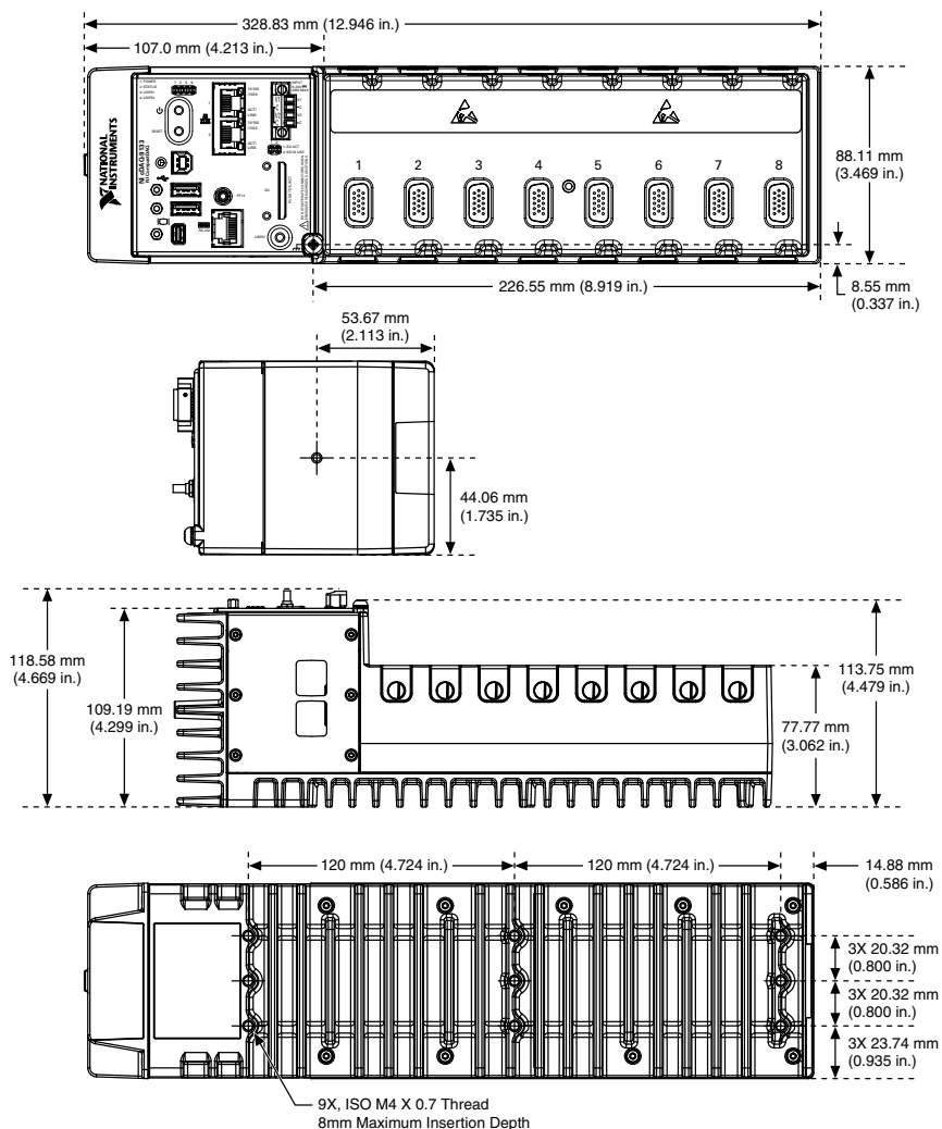
Figure 1. NI cDAQ-9133 Dimensions
