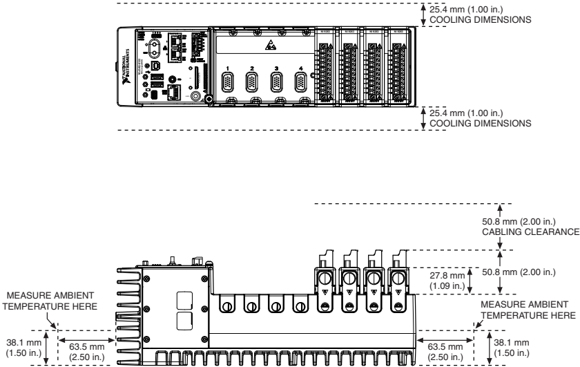
Figure 2. NI cDAQ-9133 Temperature, Cooling, and Cabling Dimensions
