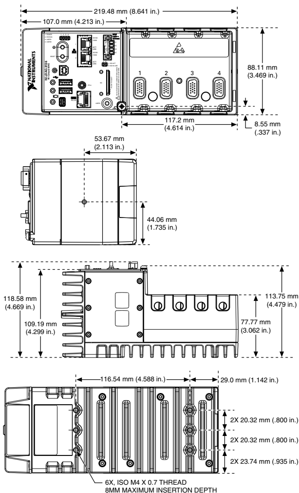
Figure 1. NI cDAQ-9134 Dimensions
