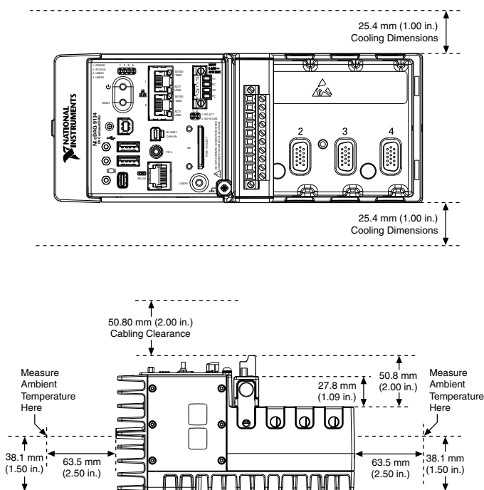
Figure 2. NI cDAQ-9134 Temperature, Cooling, and Cabling Dimensions
