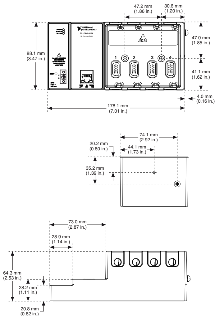
Figure 1. NI cDAQ-9184 Dimensions
