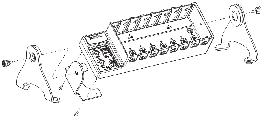
Figure 1-6. NI 9901 Desktop Mounting Kit
