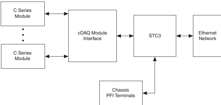
Figure 1-11. Block Diagram
