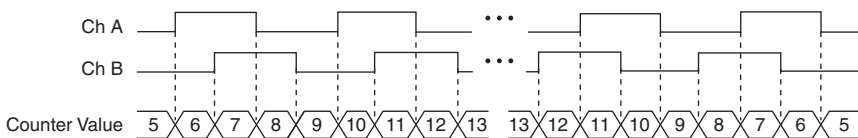
Figure 5-19. X4 Encoding
