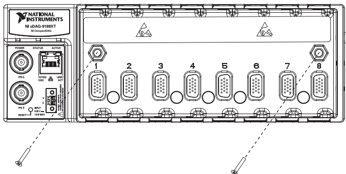
Figure 1-8. Mounting the cDAQ-9188XT Directly on a Flat Surface
