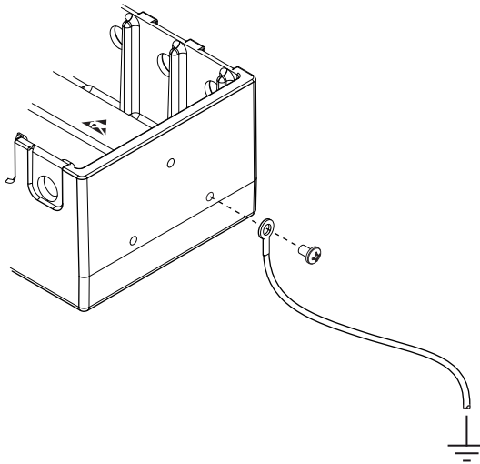
Figure 1-2. Ring Lug Attached to Chassis Ground Terminal
