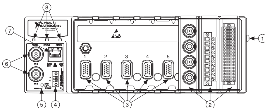
Figure 1-1. NI cDAQ-9188XT Chassis
