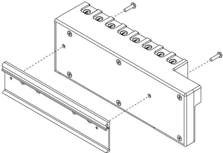
Figure 1-9. cDAQ-9188XT DIN Rail Installation
