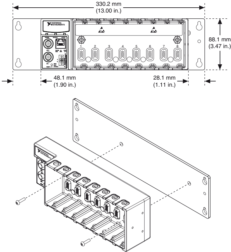
Figure 1-7. cDAQ-9188XT Panel Mount Dimensions and Installation
