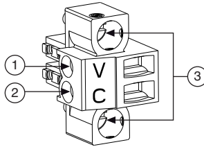
Figure 1-4. Power Screw Terminal Connector Plug
