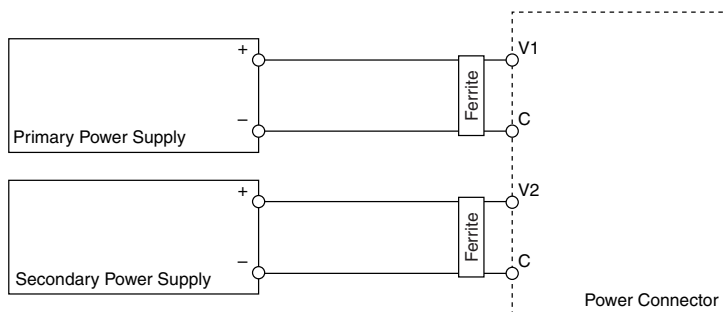
Figure 4. cRIO-9031 Power Connections
