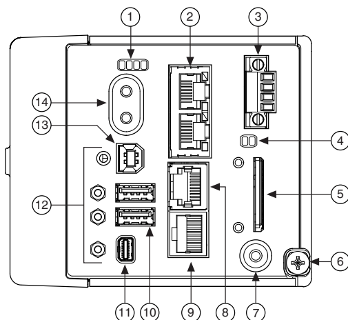
Figure 2. cRIO-9031 Front Panel
