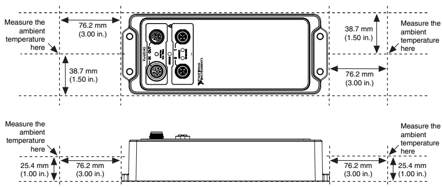
Figure 34. Ambient Temperature Locations, Horizontal Mounting Configuration
