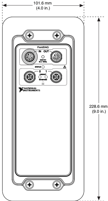
Figure 40. FD-11960 Dimensions
