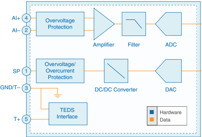
Figure 8. FD-11601 Input Circuitry
