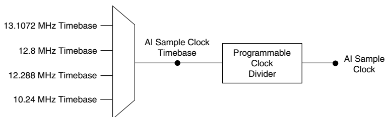
Figure 21. AI Sample Clock Timing Options
