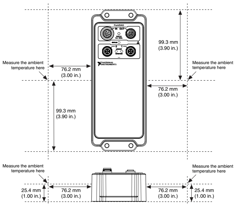
Figure 35. Ambient Temperature Locations, Vertical Mounting Configuration
