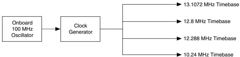
Figure 22. Clock Routing Circuitry
