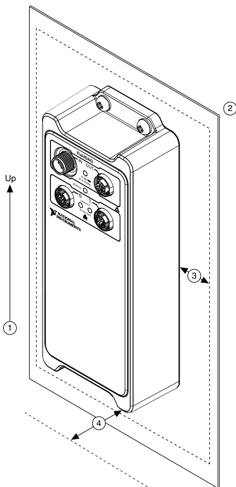
Figure 31. Reference Mounting Configuration
