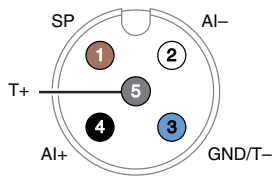
Figure 10. FD-11601 Pinout
