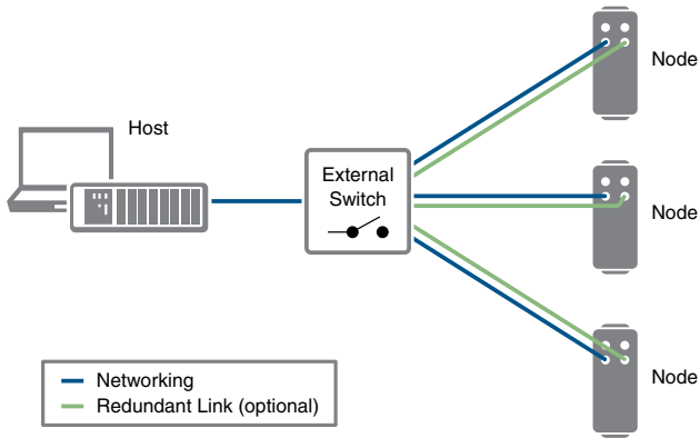
Figure 26. Star Topology
