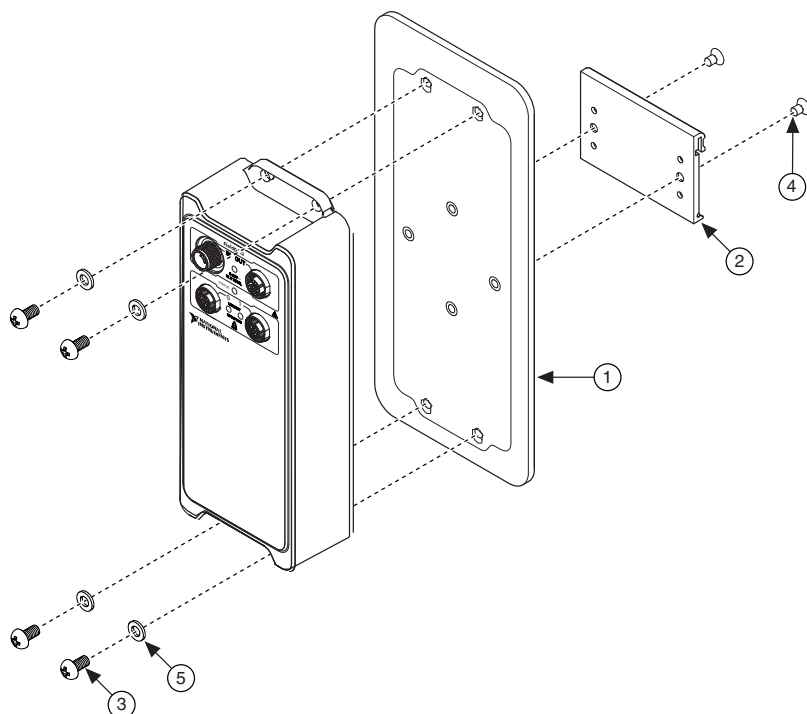
Figure 38. Attaching a FieldDAQ Device to the Bracket and DIN Rail Clip
