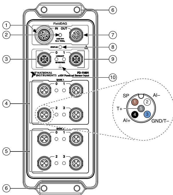
Figure 1. FD-11601 Front Panel
