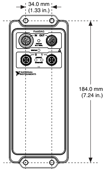
Figure 36. Surface Mounting Dimensions
