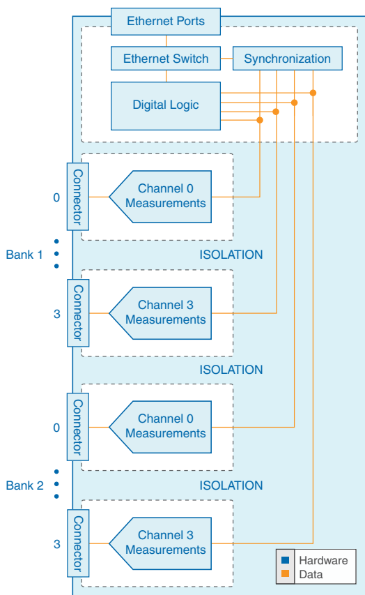
Figure 9. FD-11601 Block Diagram
