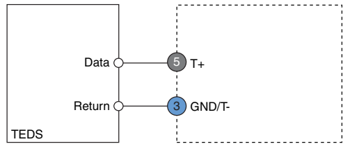
Figure 15. Connecting TEDS Sensors to the FieldDAQ Device
