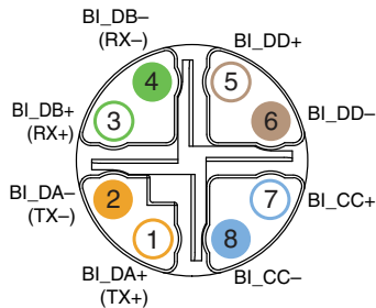
Figure 23. Ethernet Connector Pinout
