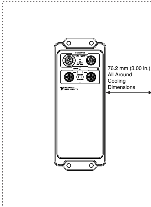
Figure 32. Cooling Dimensions
