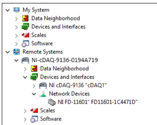
Figure 28. Adding the FieldDAQ Device to the Real-Time Controller in MAX
