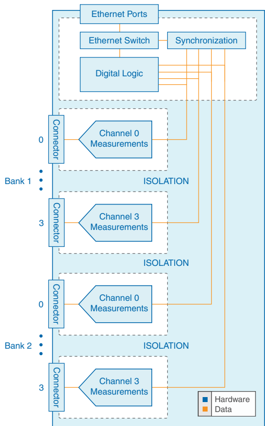
Figure 9. FD-11603 Block Diagram
