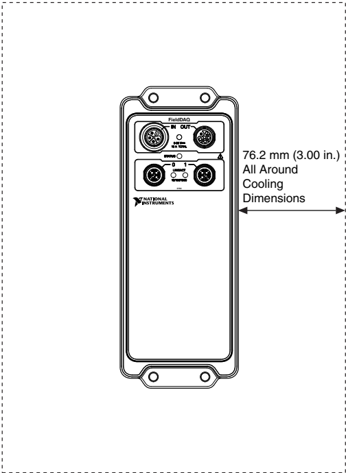
Figure 25. Cooling Dimensions
