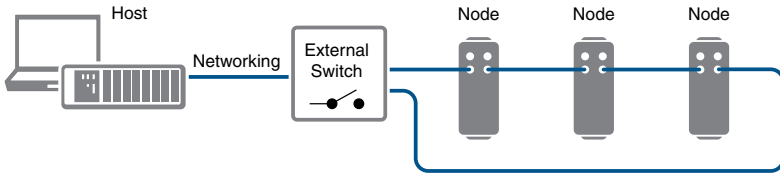
Figure 19. Ring Topology
