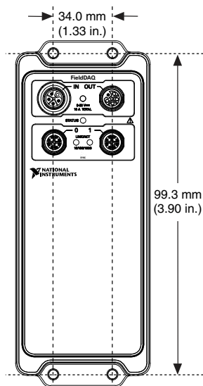
Figure 29. Surface Mounting Dimensions
