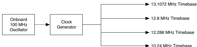
Figure 16. Clock Routing Circuitry
