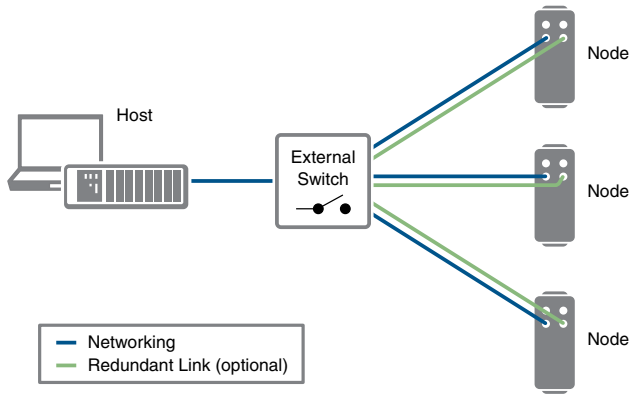
Figure 20. Star Topology
