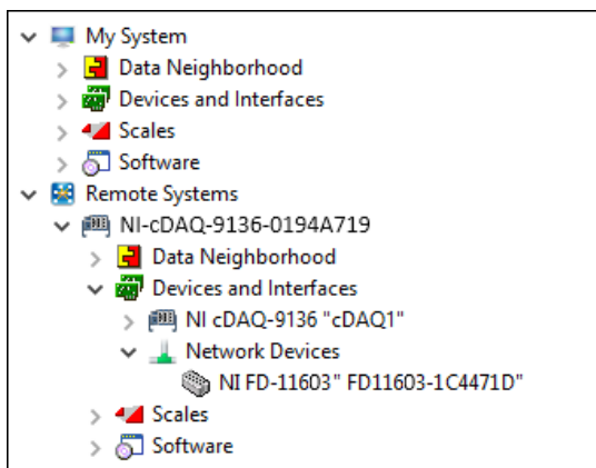
Figure 21. Adding the FieldDAQ Device to the Real-Time Controller in MAX
