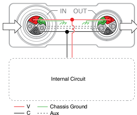
Figure 6. Power Circuitry
