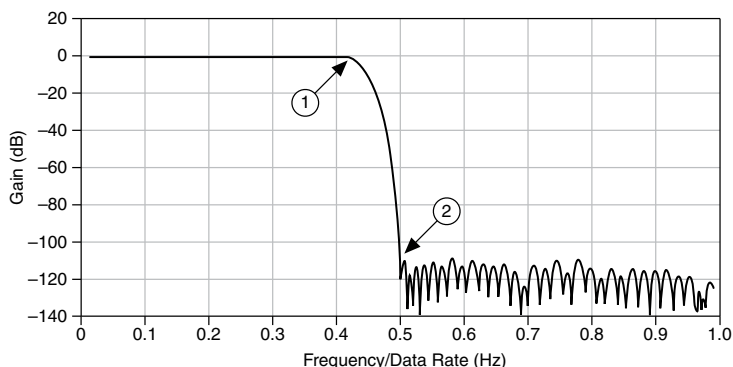
Figure 14. Transition Band and Stopband
