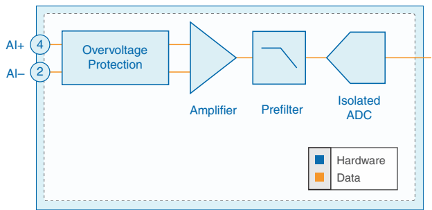
Figure 9. FD-11603 Block Diagram
