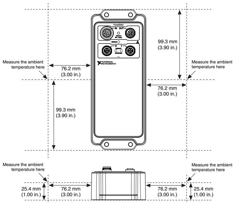
Figure 28. Ambient Temperature Locations, Vertical Mounting Configuration
