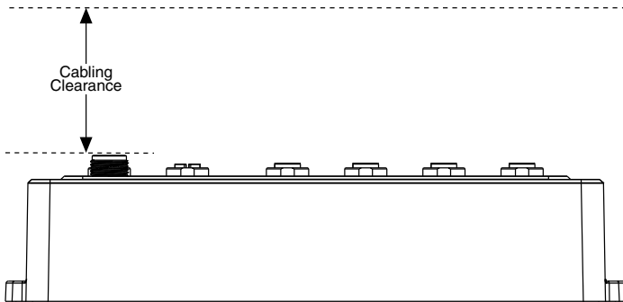
Figure 26. Cabling Clearance
