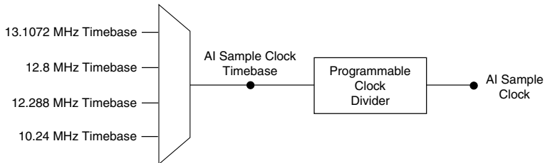
Figure 15. AI Sample Clock Timing Options
