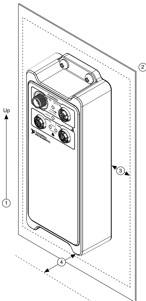
Figure 24. Reference Mounting Configuration
