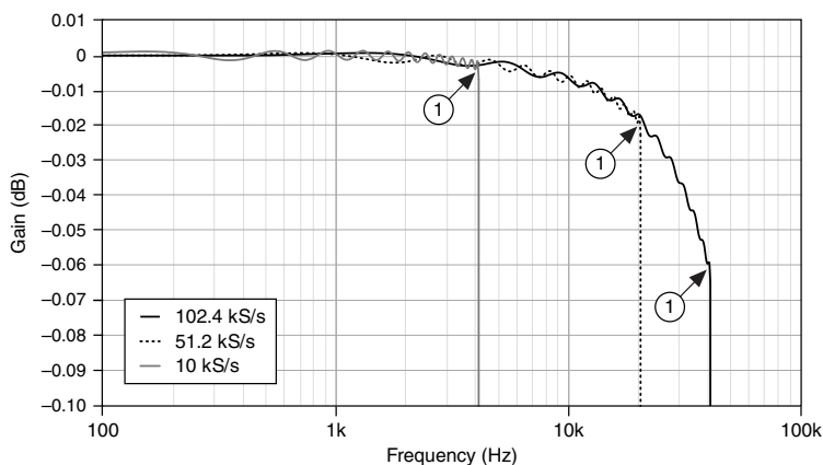
Figure 13. Typical Passband Flatness
