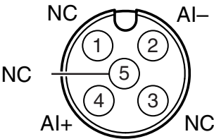
Figure 10. FD-11603 Pinout
