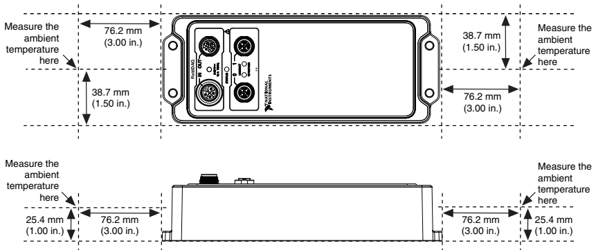
Figure 27. Ambient Temperature Locations, Horizontal Mounting Configuration
