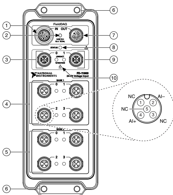
Figure 1. FD-11603 Front Panel
