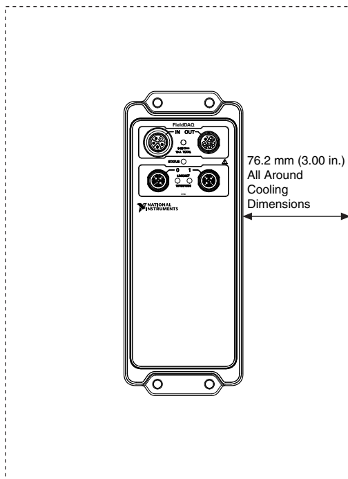
Figure 33. Cooling Dimensions
