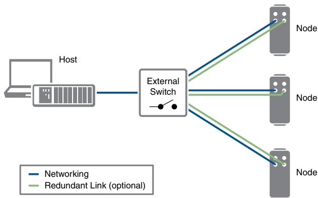
Figure 17. Star Topology
