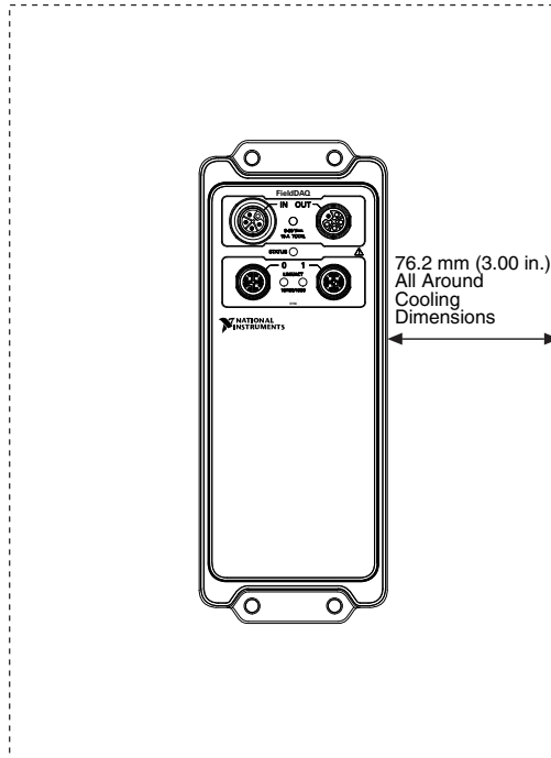
Figure 22. Cooling Dimensions
