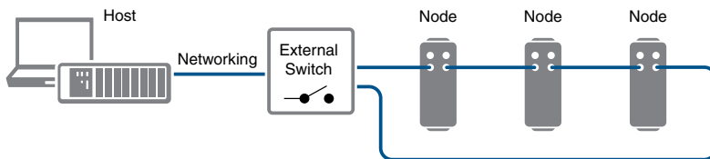
Figure 17. Ring Topology
