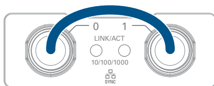
Figure 22. Connecting Port 0 and Port 1
