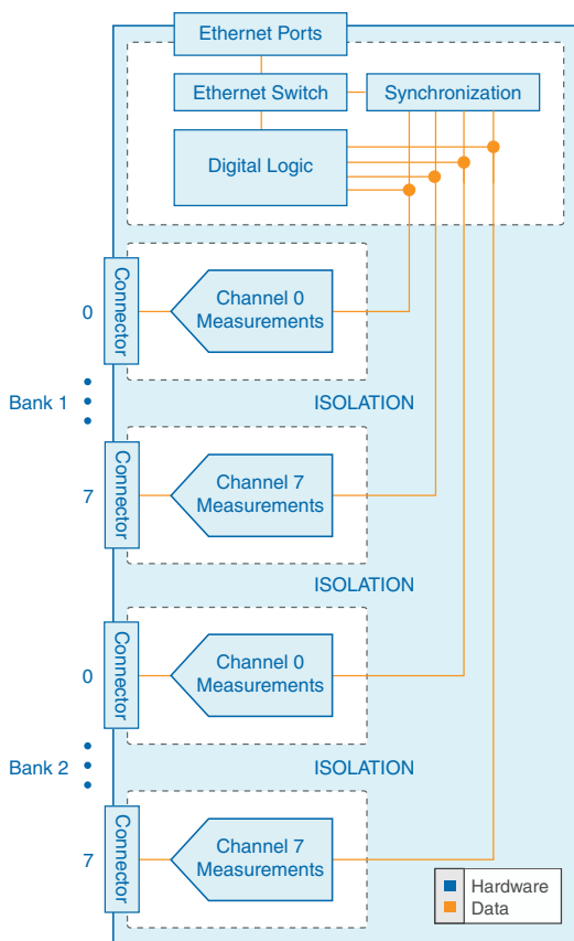
Figure 9. FD-11614 Block Diagram
