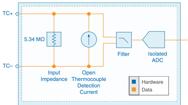
Figure 8. FD-11614 Input Circuitry
