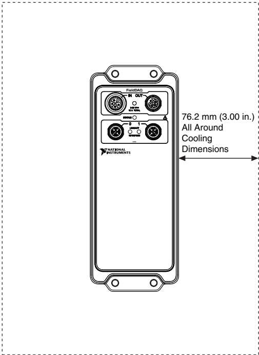
Figure 24. Cooling Dimensions
