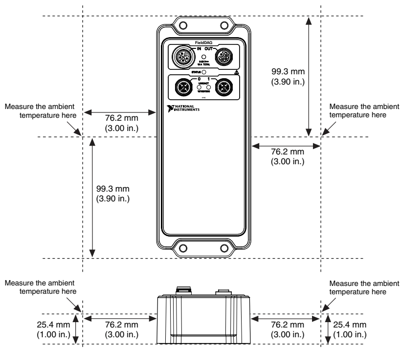
Figure 27. Ambient Temperature Locations, Vertical Mounting Configuration
