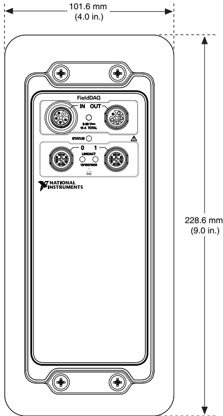
Figure 32. FD-11960 Dimensions
