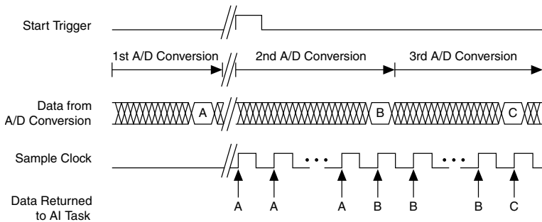
Figure 13. Sample Clock Timing Example
