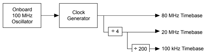
Figure 14. Clock Routing Circuitry
