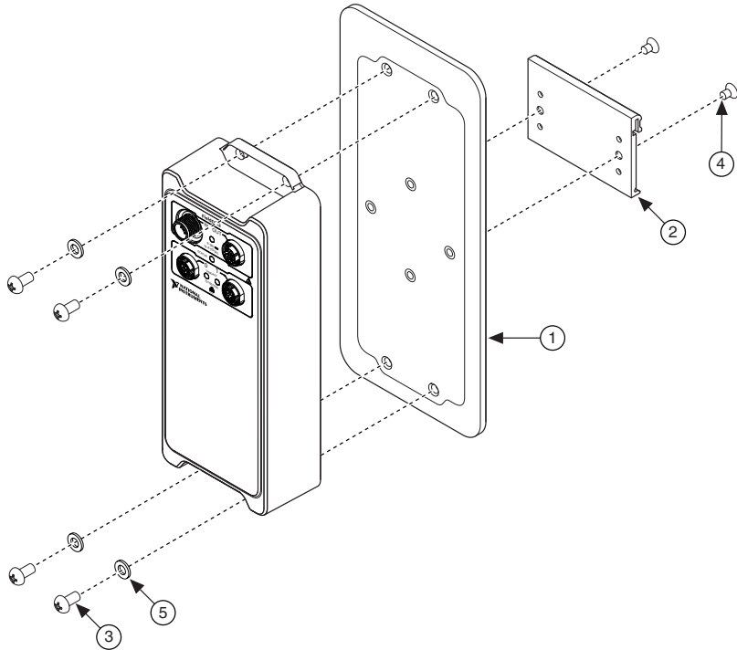
Figure 30. Attaching a FieldDAQ Device to the Bracket and DIN Rail Clip
