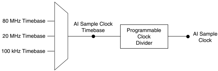
Figure 12. AI Sample Clock Timing Options
