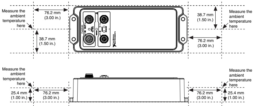
Figure 26. Ambient Temperature Locations, Horizontal Mounting Configuration
