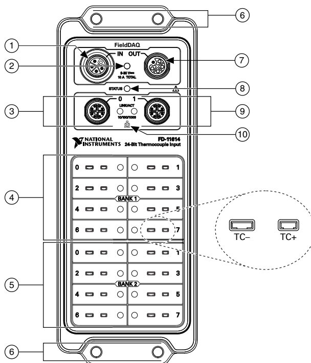
Figure 1. FD-11614 Front Panel
