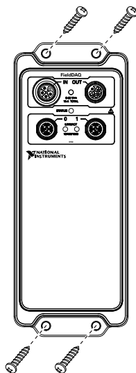
Figure 29. Fastening the Device to the Surface
