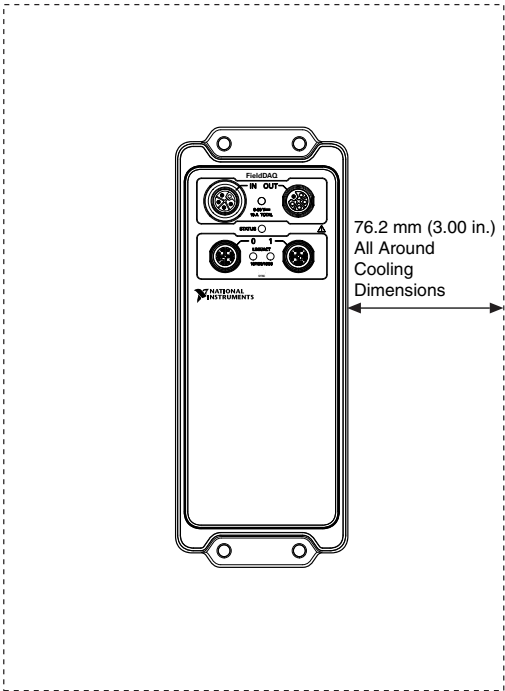
Figure 30. Cooling Dimensions
