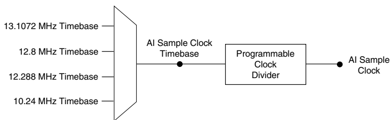
Figure 19. AI Sample Clock Timing Options
