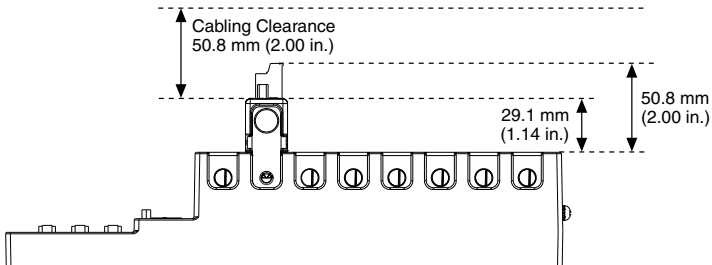
Figure 6. CMS/MMS-9068 Cabling Clearance
