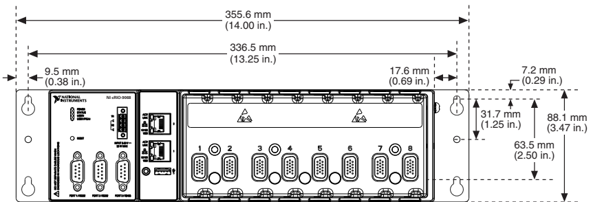
Figure 9. CMS/MMS-9068 Panel Mounting Dimensions
