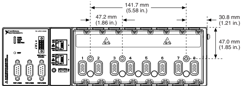
Figure 8. CMS/MMS-9068 Surface Mounting Dimensions
