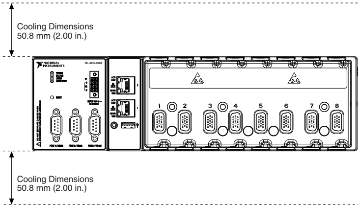
Figure 5. CMS/MMS-9068 Cooling Dimensions
