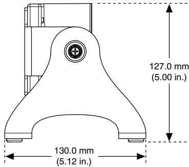
Figure 11. CMS/MMS-9068 Desktop Mounting Side Dimensions
