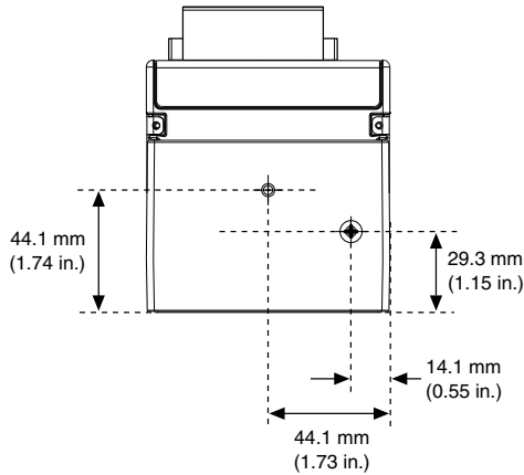
Figure 4. CMS/MMS-9068 Side Dimensions
