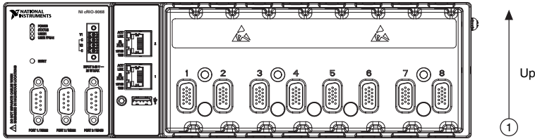
Figure 2. CMS/MMS-9068 Horizontal Mounting
