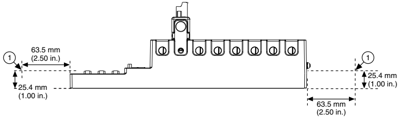
Figure 7. CMS/MMS-9068 Ambient Temperature Location
