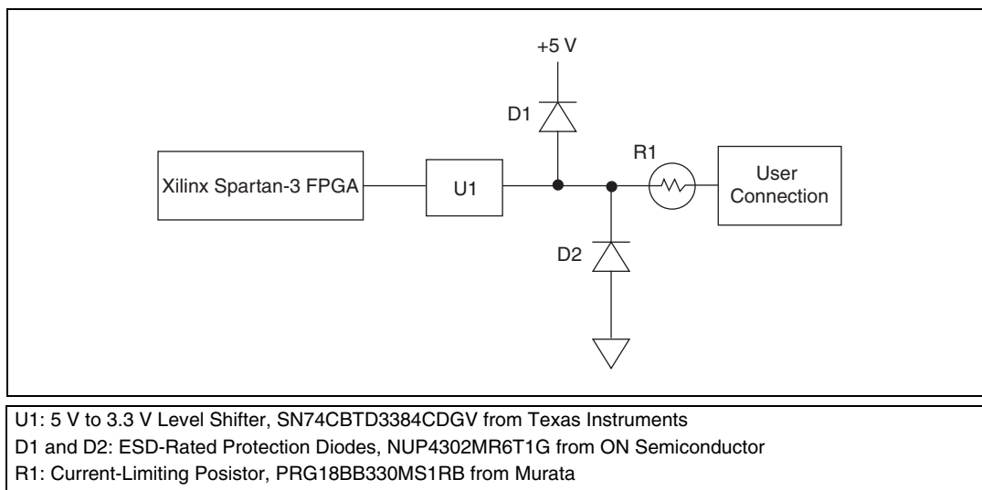
Figure 13. Circuitry of One 3.3 V DIO Channel
