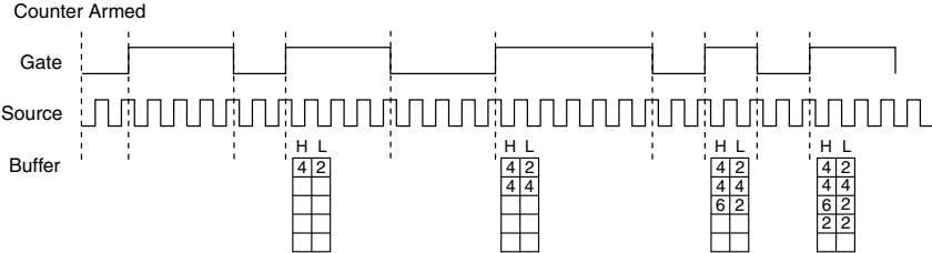
Figure 37. Implicit Buffered Pulse Measurement
