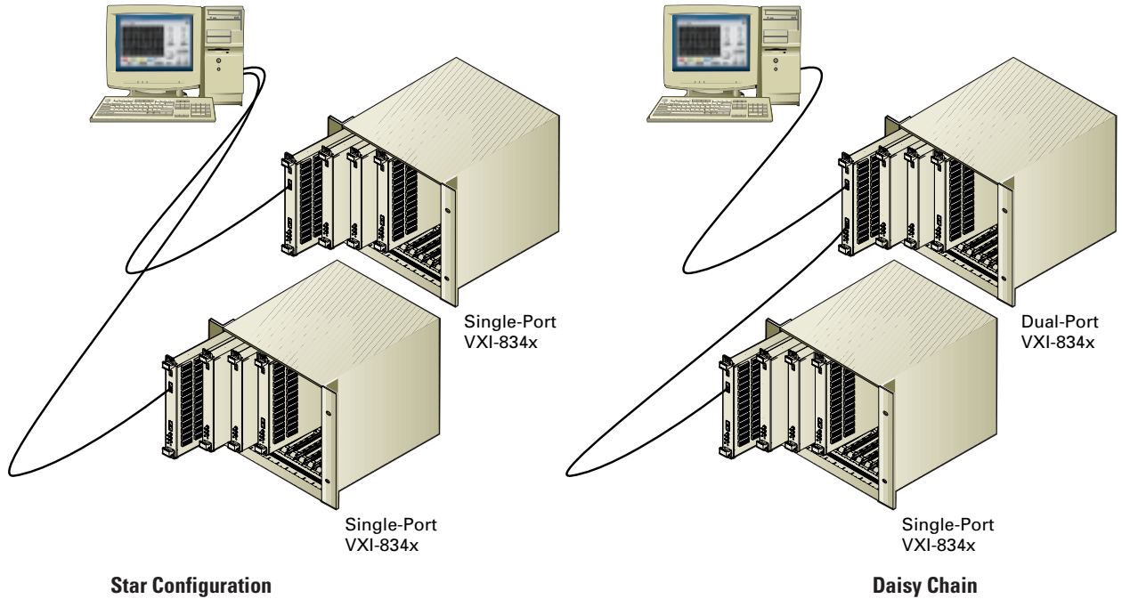
Figure 2. Multiple-Chassis VXI Configurations
